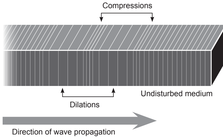
P Wave
