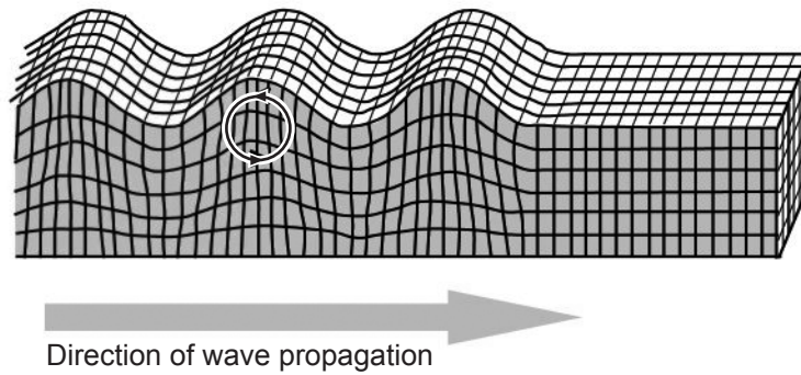
Rayleigh wave
