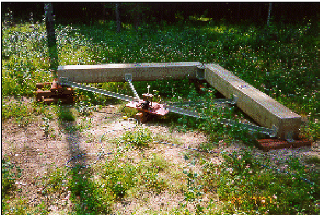
An induction magnetometer measures how fast Earth's magnetic field is changing.
